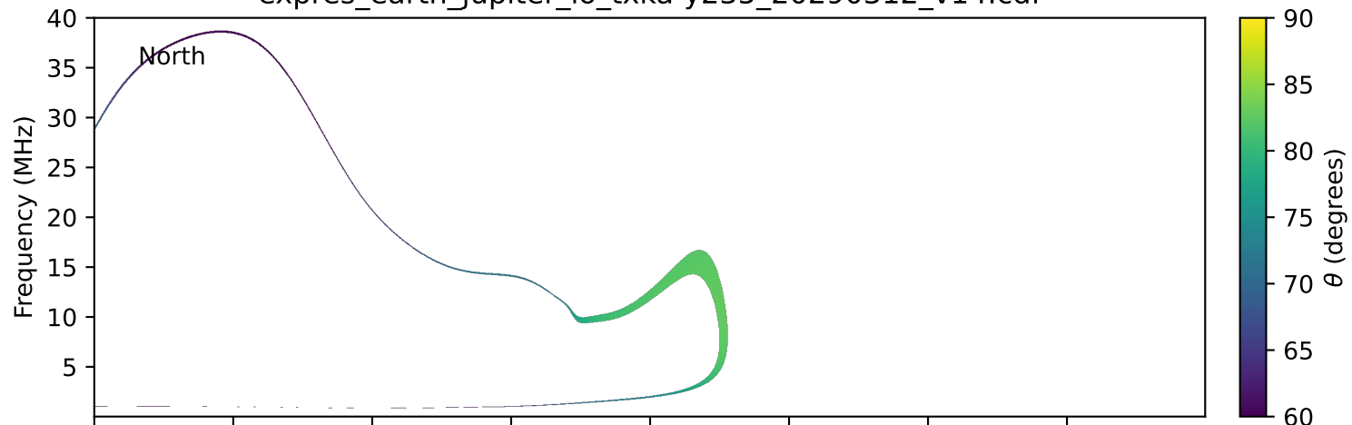
expres_earth_jupiter_io_txka-y235_20290312_v14.cdf
