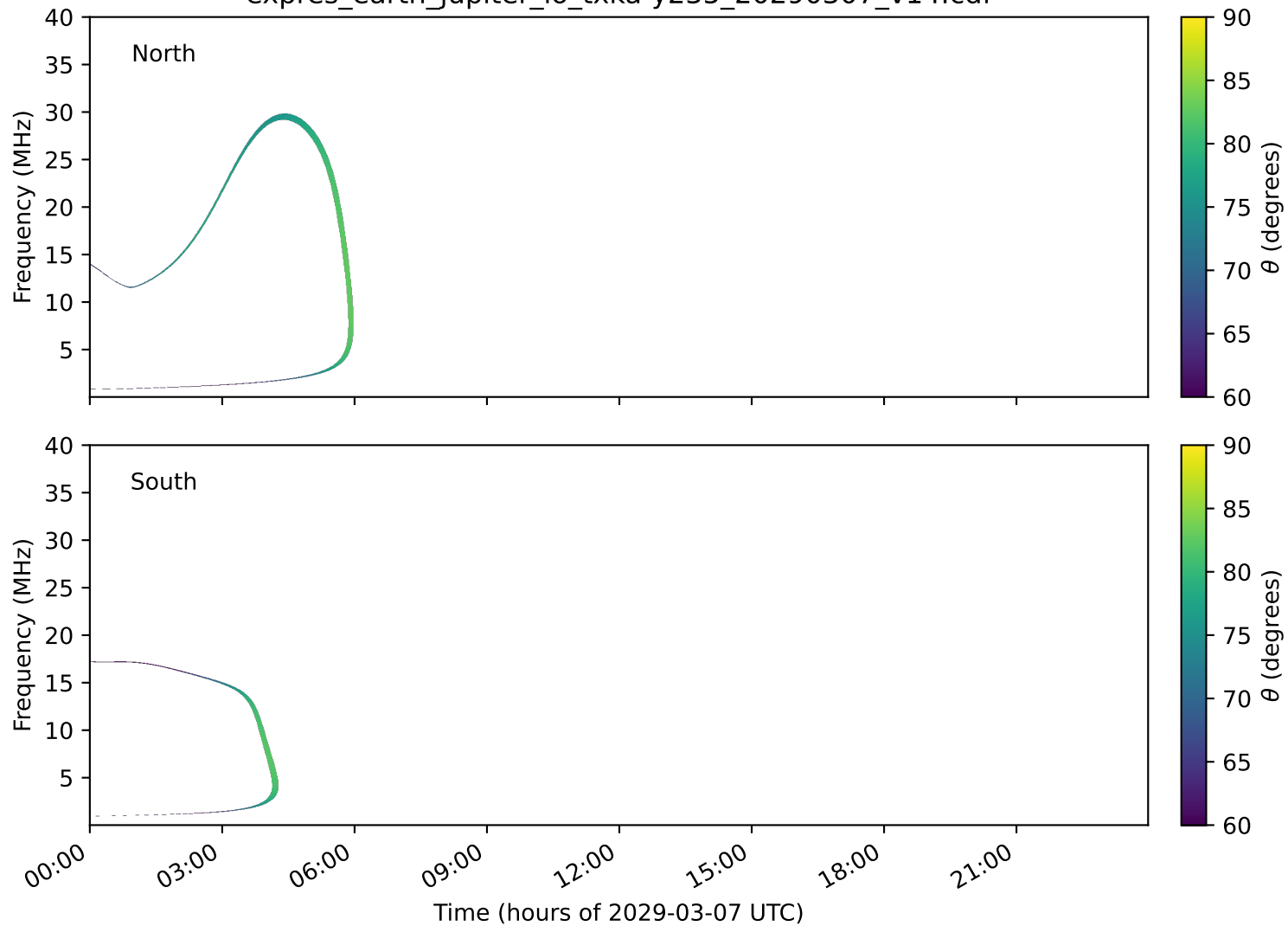
expres_earth_jupiter_io_txka-y235_20290307_v14.cdf
