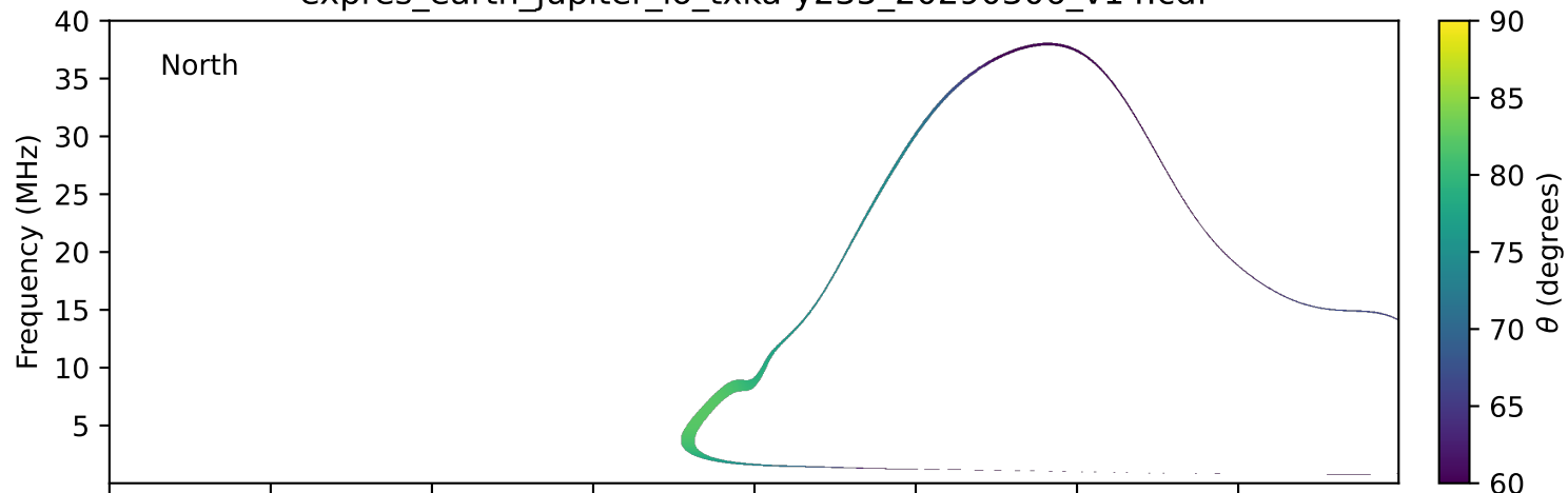
expres_earth_jupiter_io_txka-y235_20290306_v14.cdf
