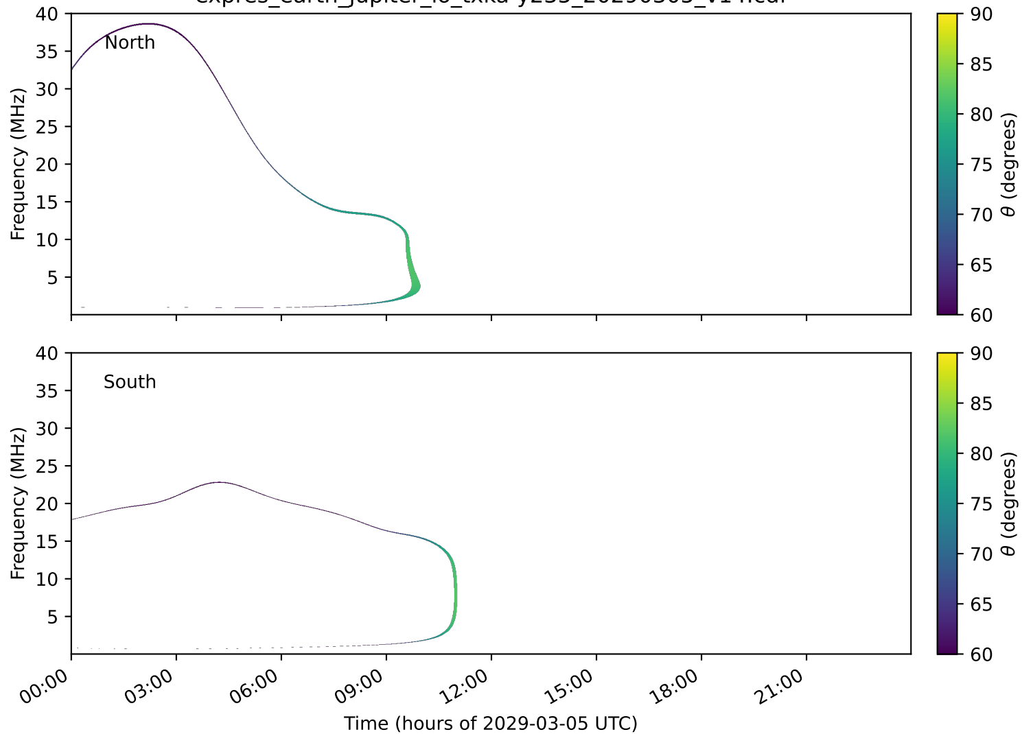
expres_earth_jupiter_io_txka-y235_20290305_v14.cdf
