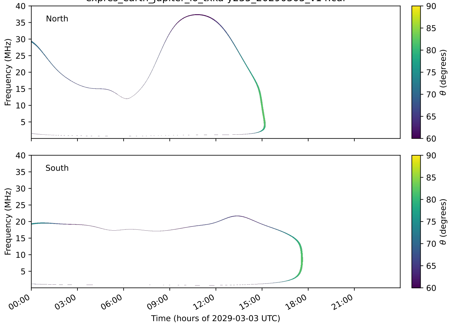
expres_earth_jupiter_io_txka-y235_20290303_v14.cdf
