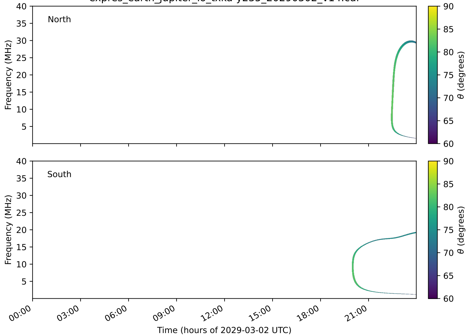
expres_earth_jupiter_io_txka-y235_20290302_v14.cdf
