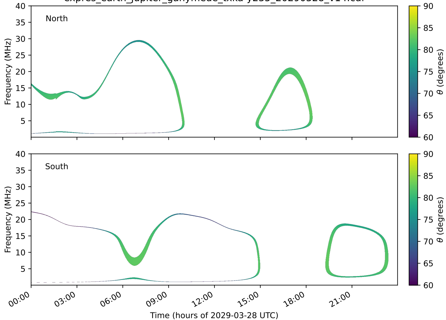
expres_earth_jupiter_ganymede_txka-y235_20290328_v14.cdf
