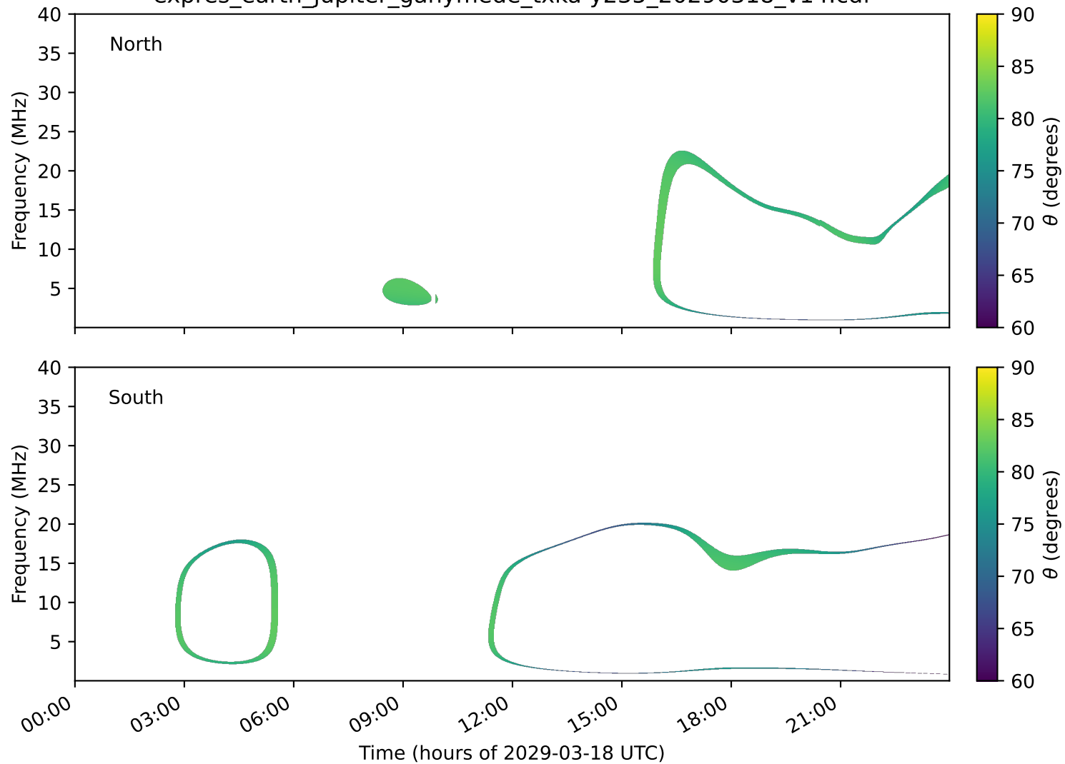
expres_earth_jupiter_ganymede_txka-y235_20290318_v14.cdf
