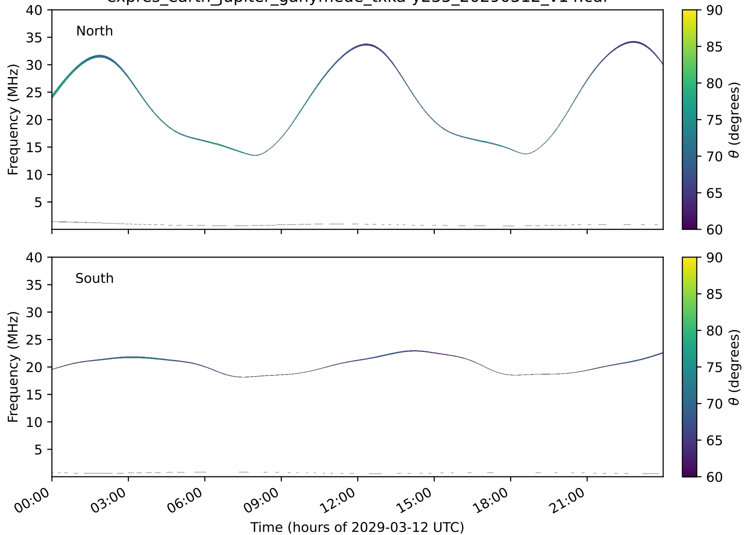
expres_earth_jupiter_ganymede_txka-y235_20290312_v14.cdf
