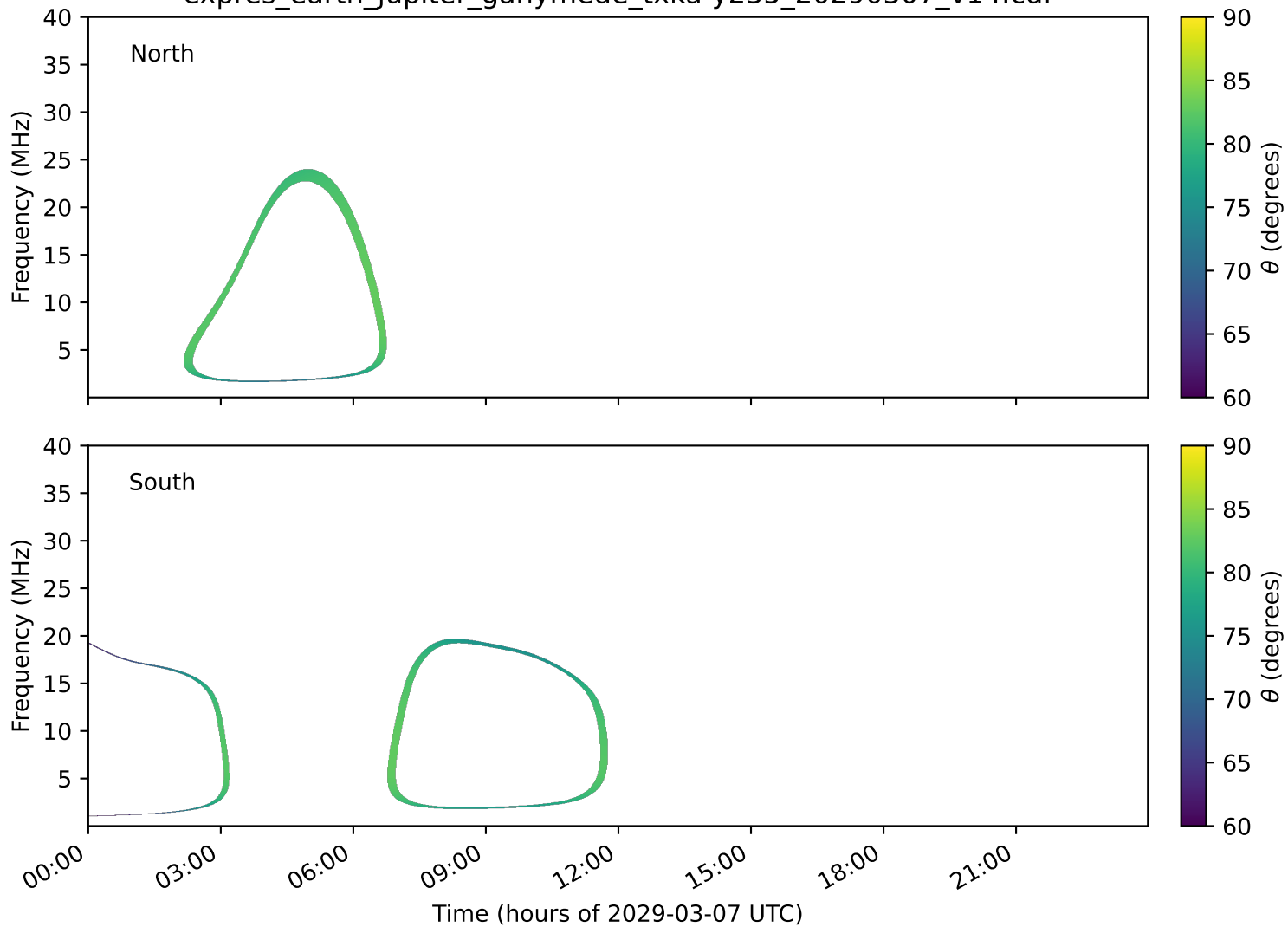
expres_earth_jupiter_ganymede_txka-y235_20290307_v14.cdf
