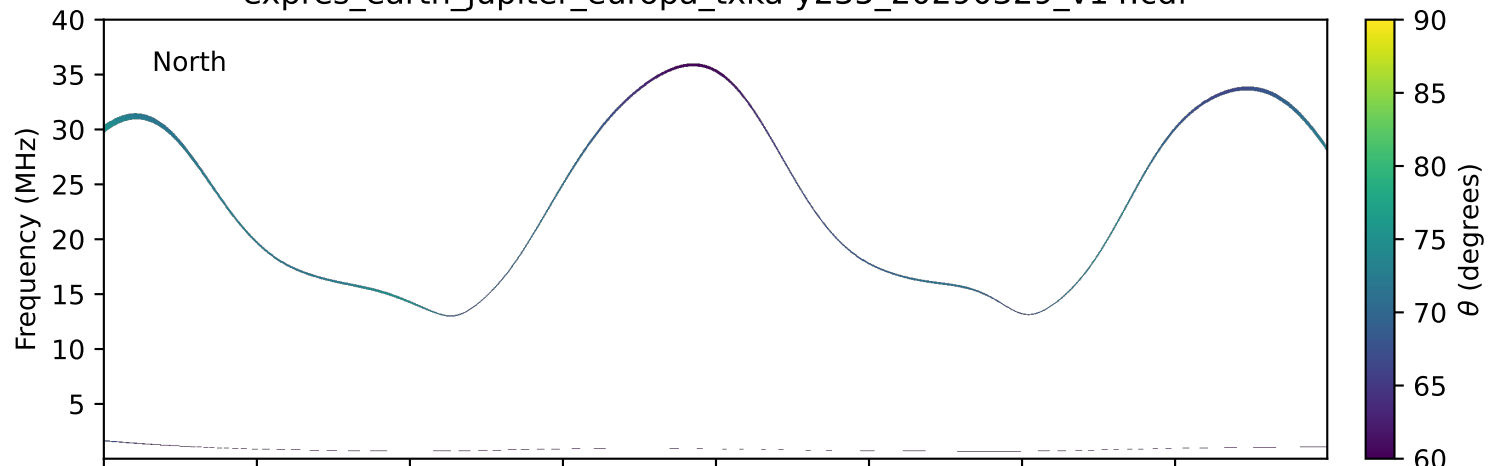
expres_earth_jupiter_europa_txka-y235_20290329_v14.cdf
