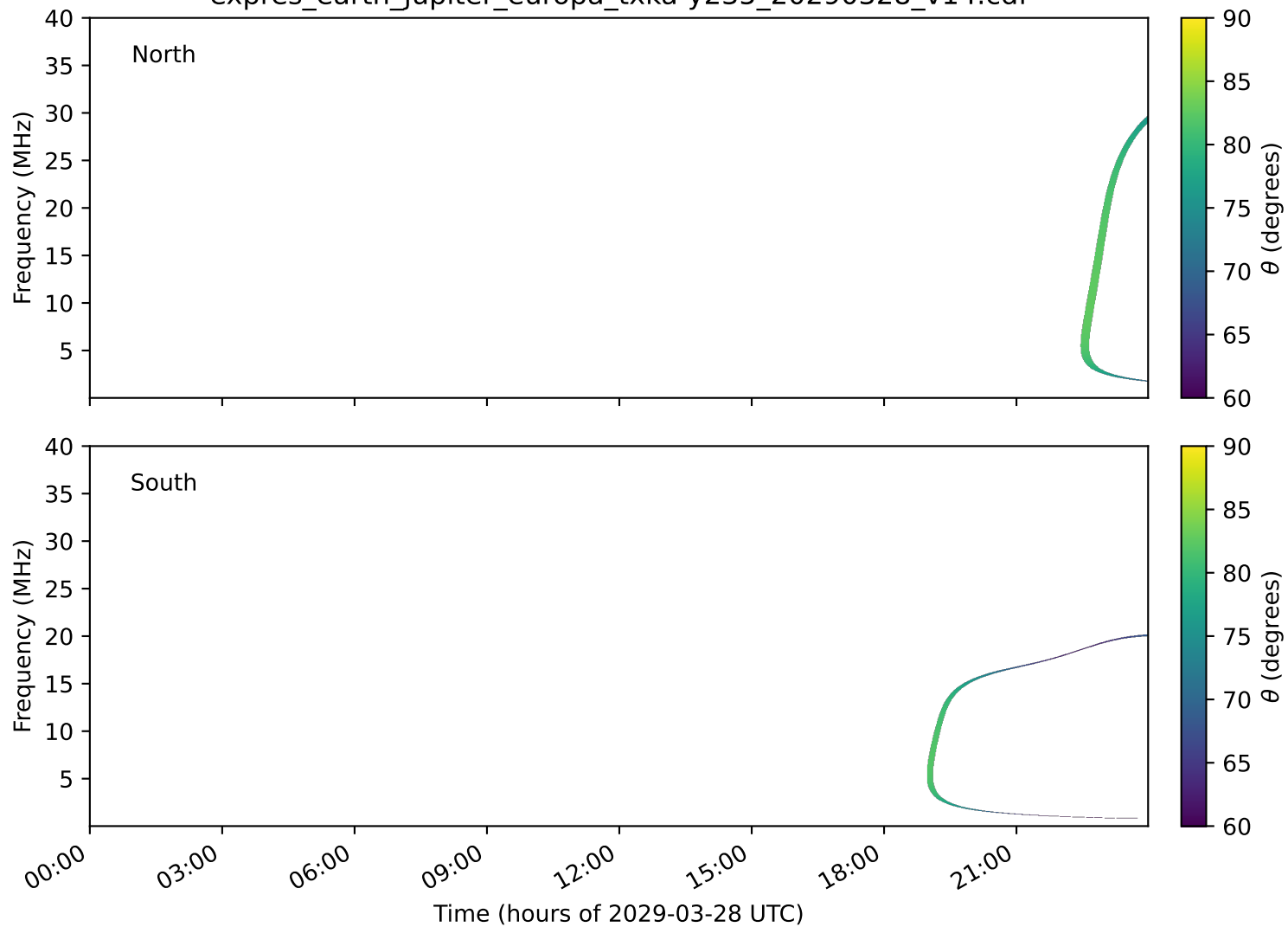
expres_earth_jupiter_europa_txka-y235_20290328_v14.cdf
