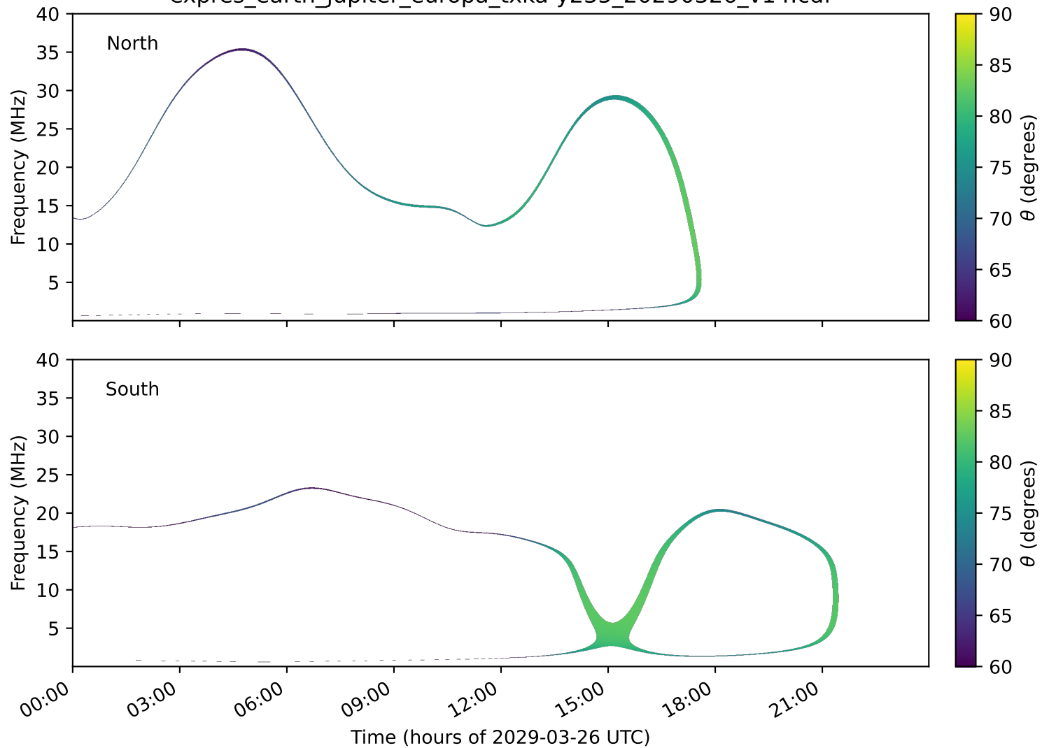
expres_earth_jupiter_europa_txka-y235_20290326_v14.cdf
