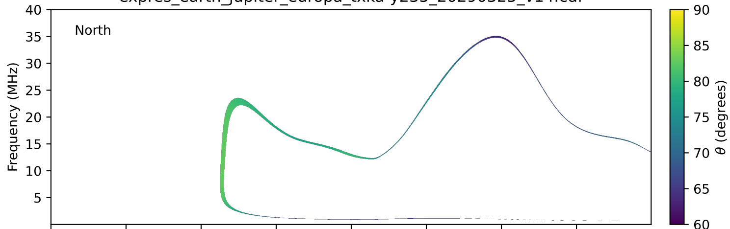
expres_earth_jupiter_europa_txka-y235_20290325_v14.cdf
