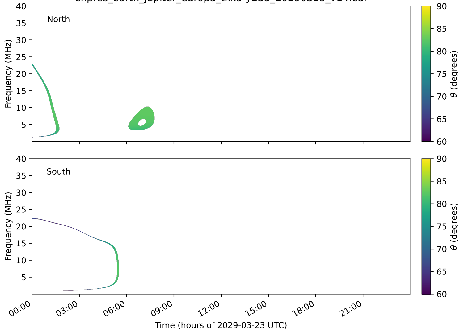
expres_earth_jupiter_europa_txka-y235_20290323_v14.cdf
