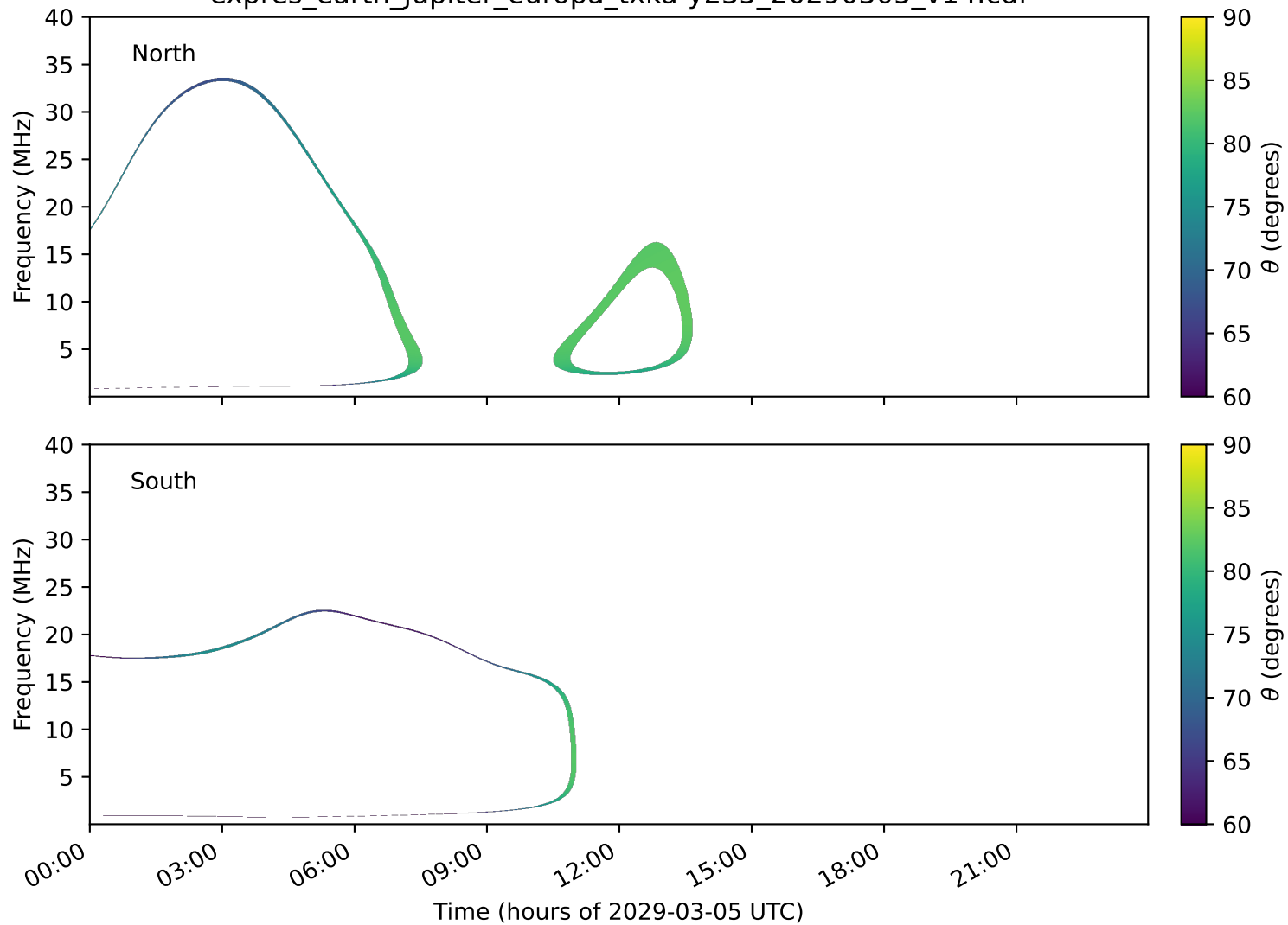
expres_earth_jupiter_europa_txka-y235_20290305_v14.cdf
