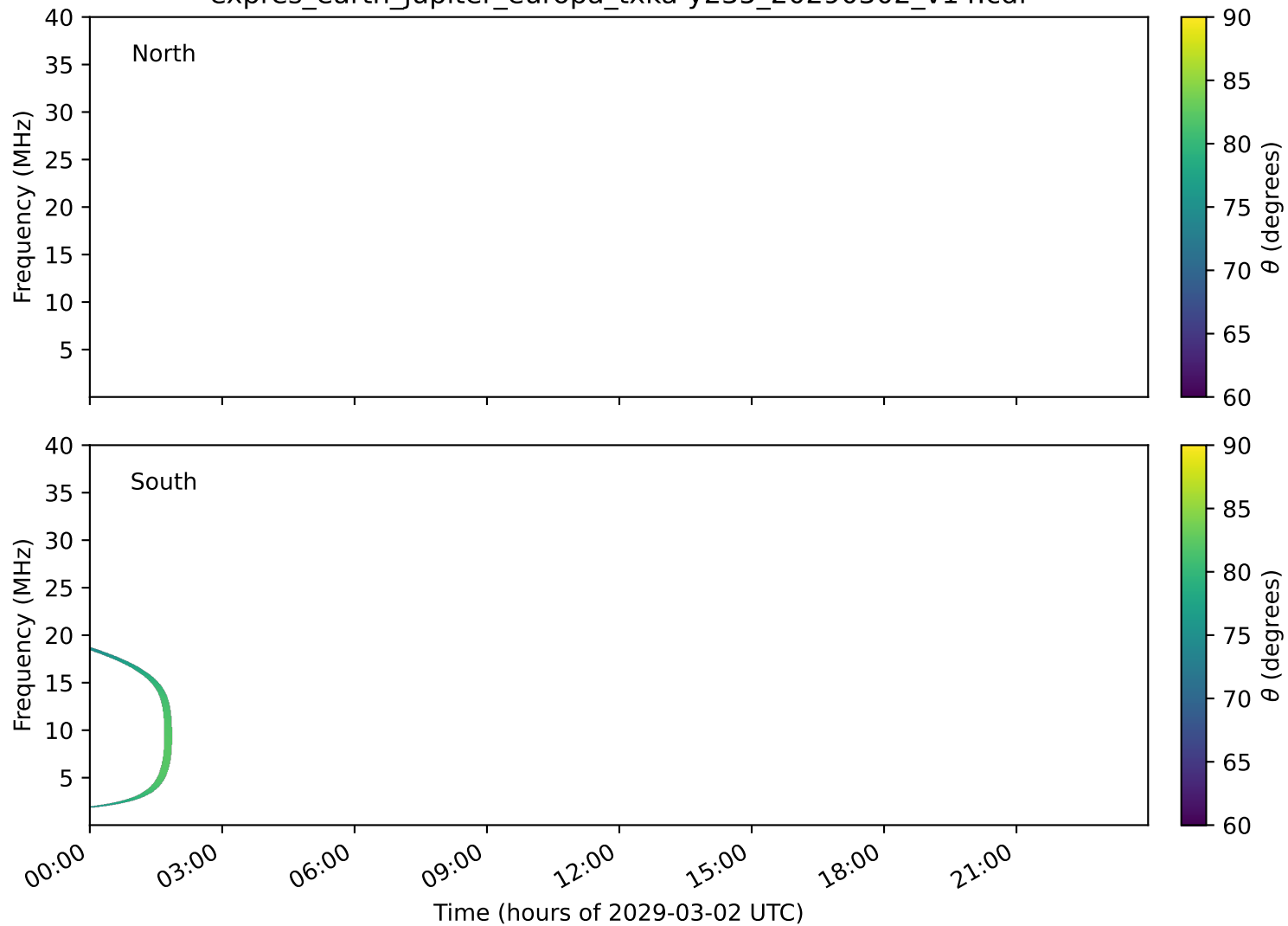
expres_earth_jupiter_europa_txka-y235_20290302_v14.cdf
