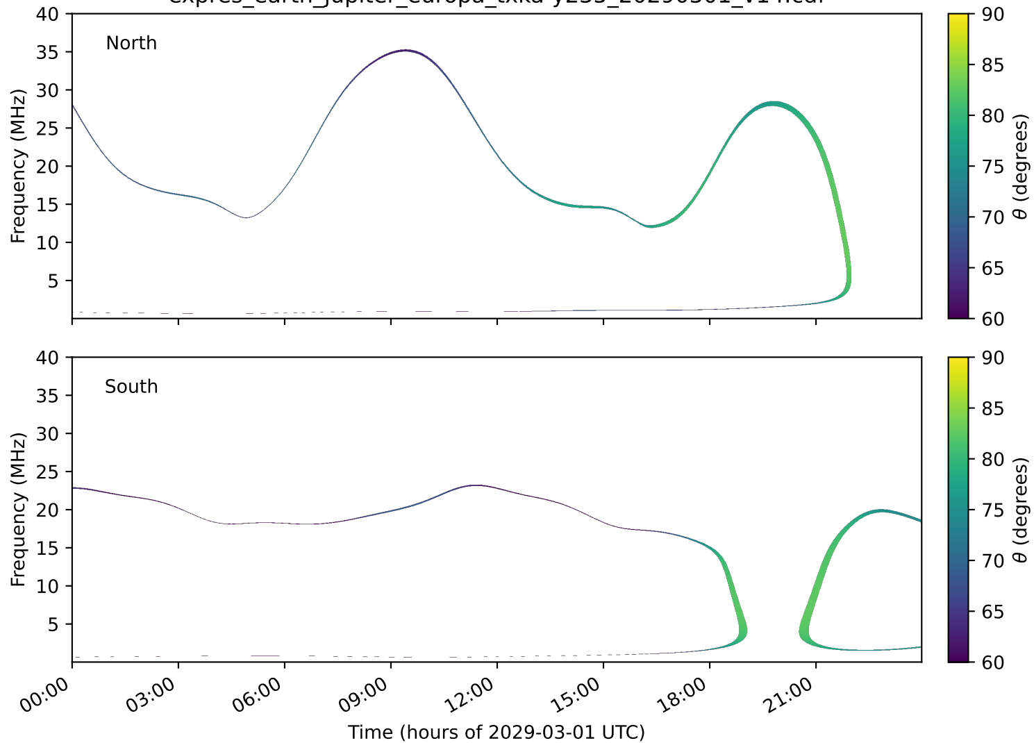
expres_earth_jupiter_europa_txka-y235_20290301_v14.cdf
