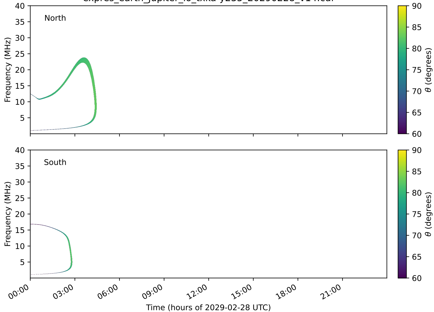
expres_earth_jupiter_io_txka-y235_20290228_v14.cdf
