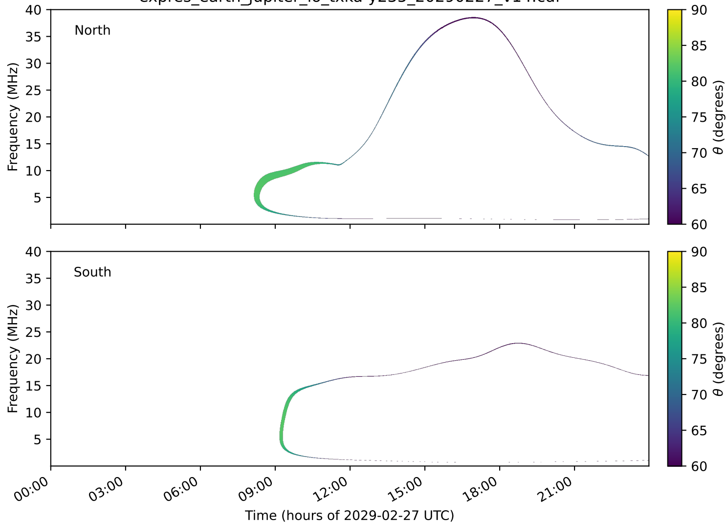
expres_earth_jupiter_io_txka-y235_20290227_v14.cdf
