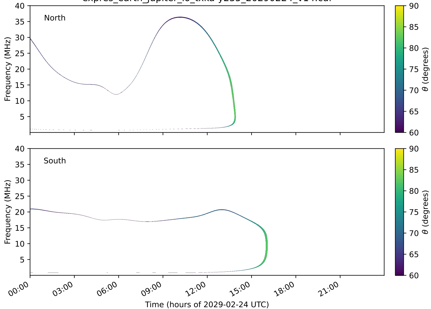
expres_earth_jupiter_io_txka-y235_20290224_v14.cdf
