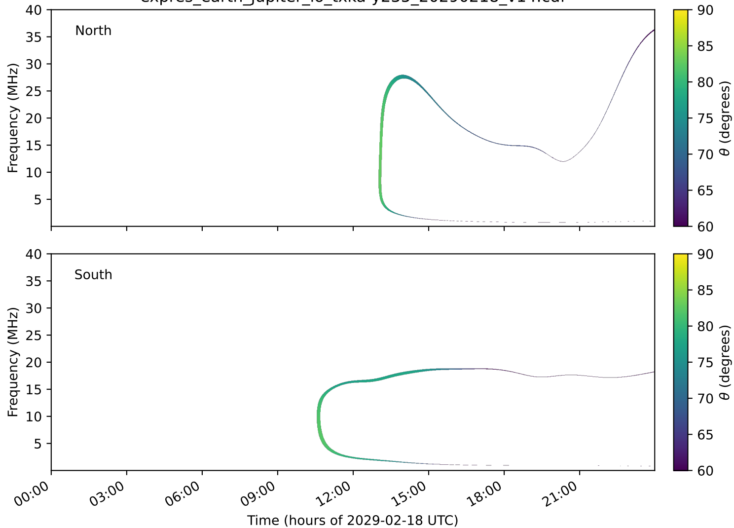
expres_earth_jupiter_io_txka-y235_20290218_v14.cdf
