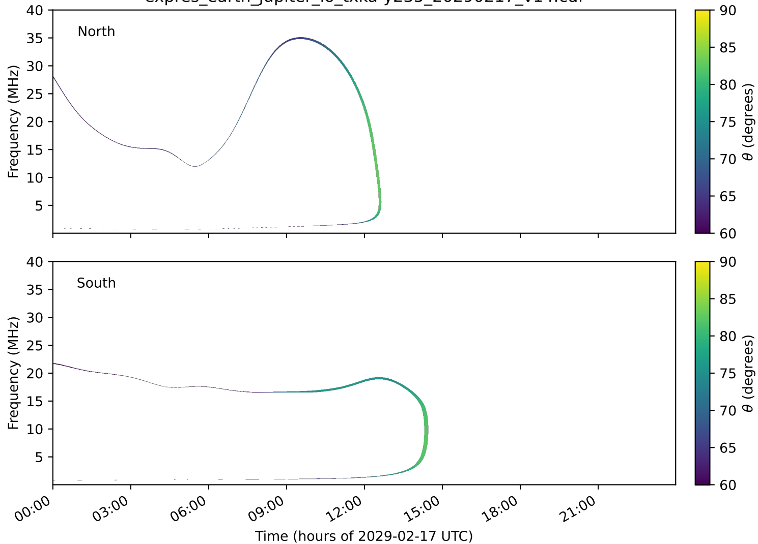
expres_earth_jupiter_io_txka-y235_20290217_v14.cdf
