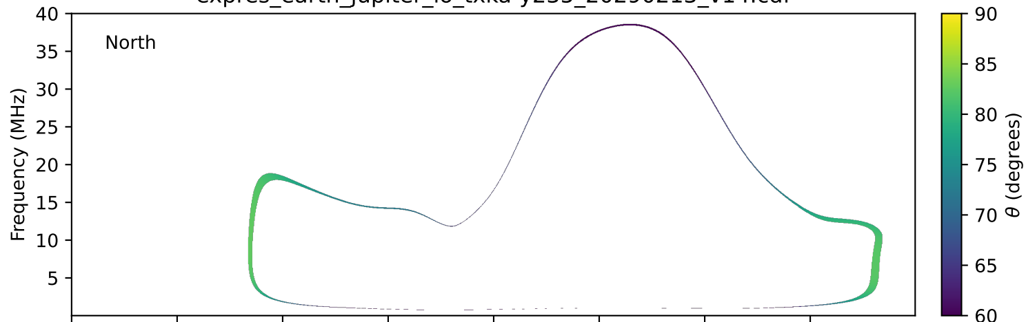
expres_earth_jupiter_io_txka-y235_20290213_v14.cdf
