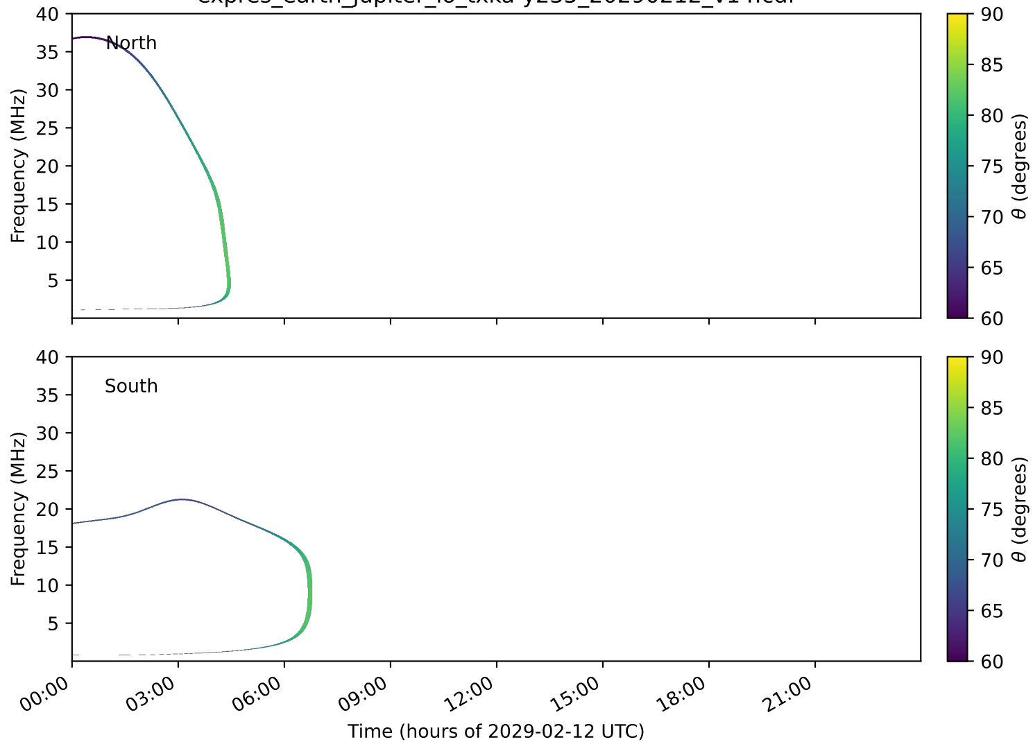
expres_earth_jupiter_io_txka-y235_20290212_v14.cdf
