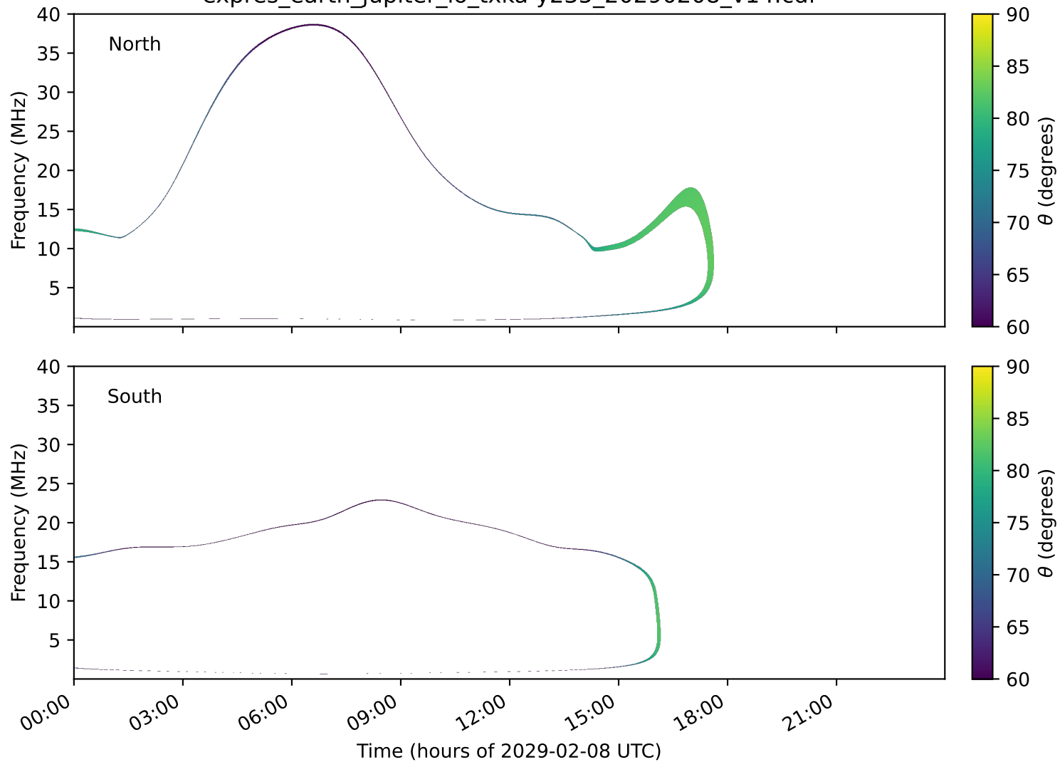
expres_earth_jupiter_io_txka-y235_20290208_v14.cdf
