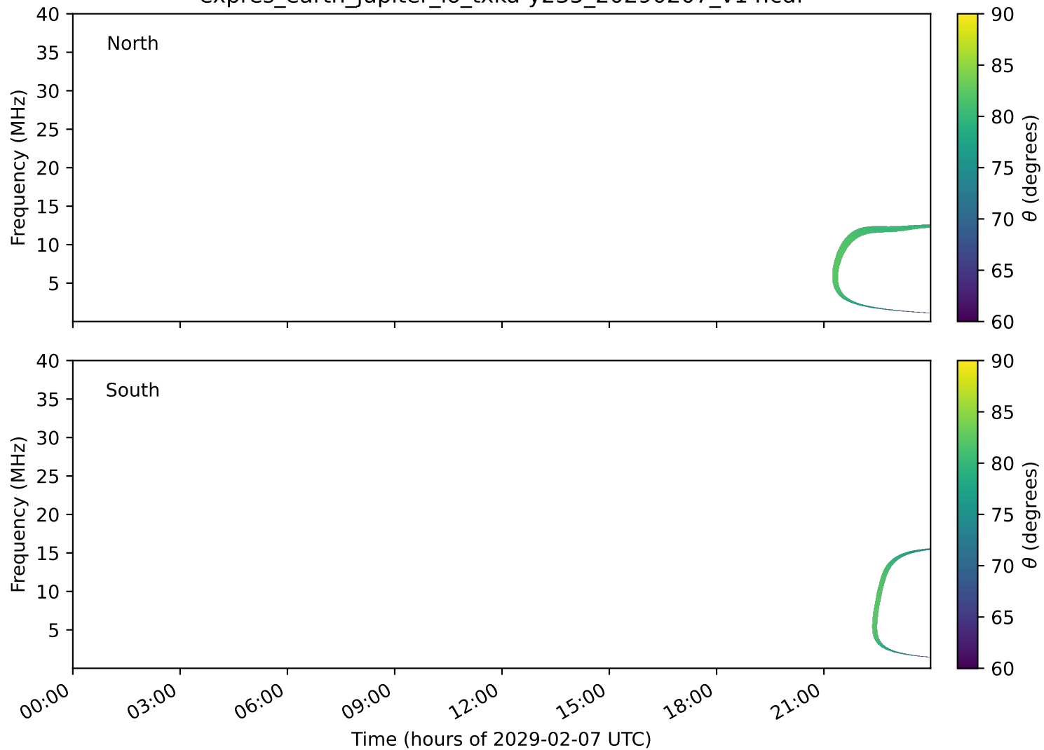
expres_earth_jupiter_io_txka-y235_20290207_v14.cdf
