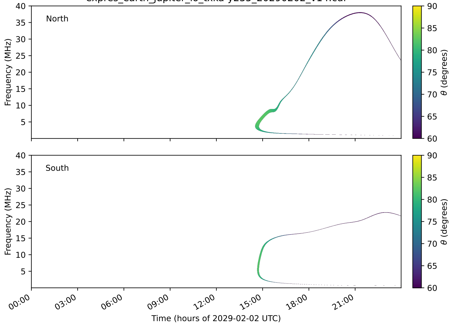
expres_earth_jupiter_io_txka-y235_20290202_v14.cdf
