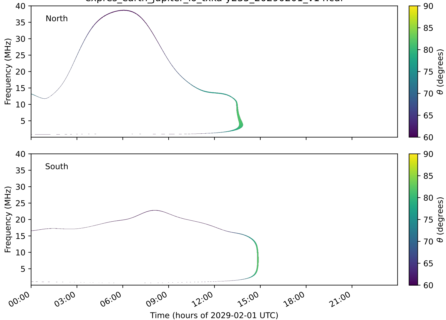
expres_earth_jupiter_io_txka-y235_20290201_v14.cdf
