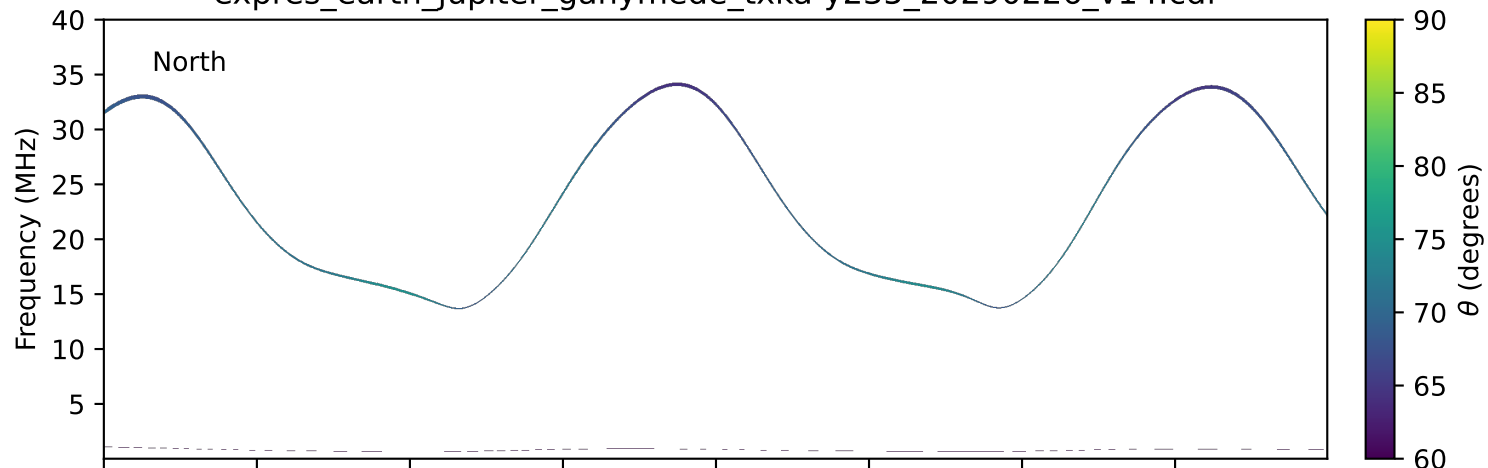
expres_earth_jupiter_ganymede_txka-y235_20290226_v14.cdf
