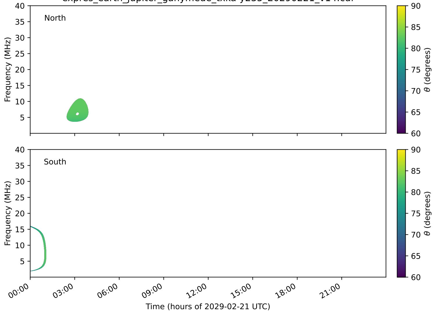
expres_earth_jupiter_ganymede_txka-y235_20290221_v14.cdf
