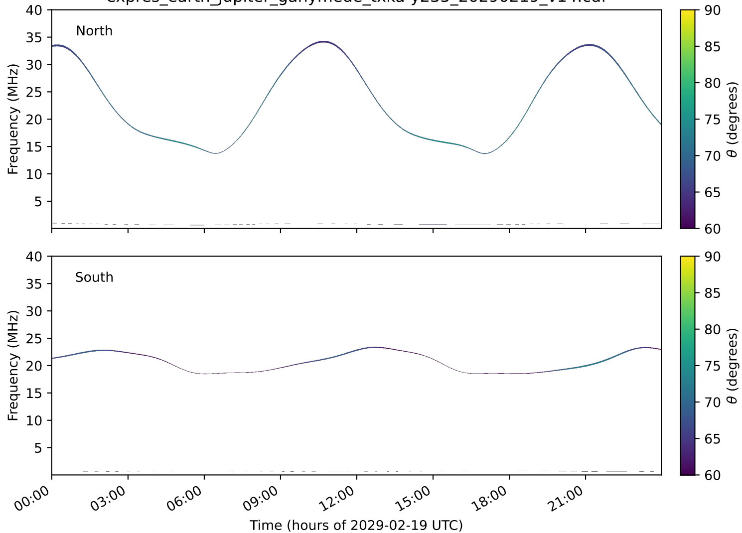
expres_earth_jupiter_ganymede_txka-y235_20290219_v14.cdf
