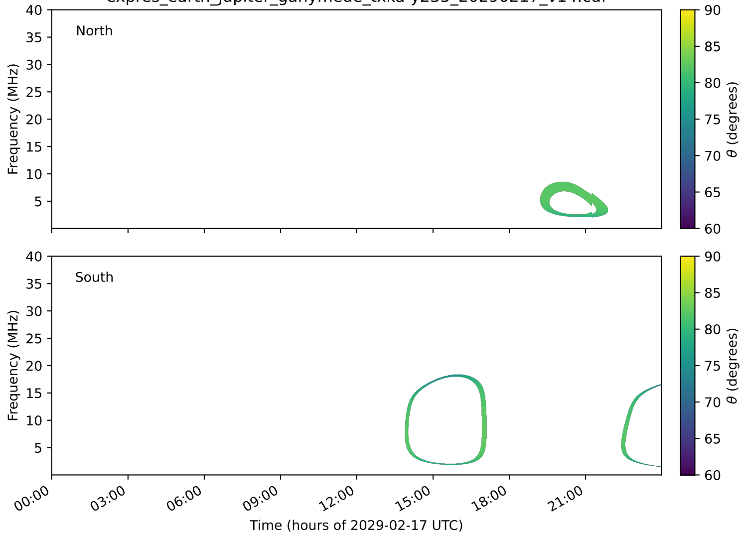
expres_earth_jupiter_ganymede_txka-y235_20290217_v14.cdf
