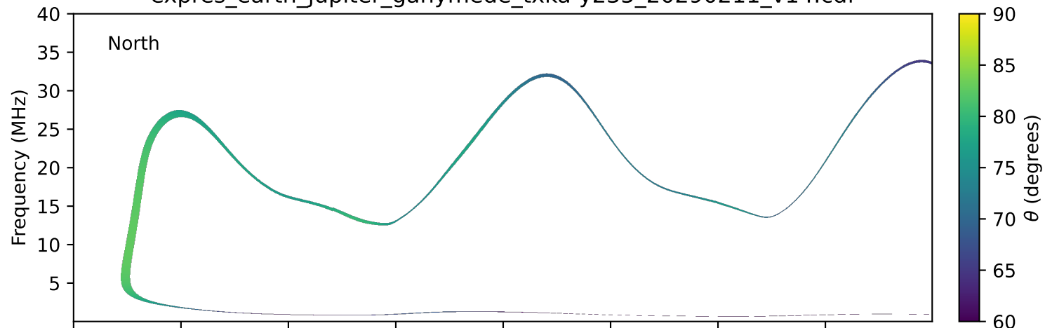
expres_earth_jupiter_ganymede_txka-y235_20290211_v14.cdf
