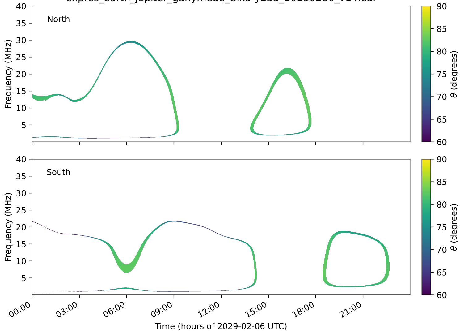
expres_earth_jupiter_ganymede_txka-y235_20290206_v14.cdf
