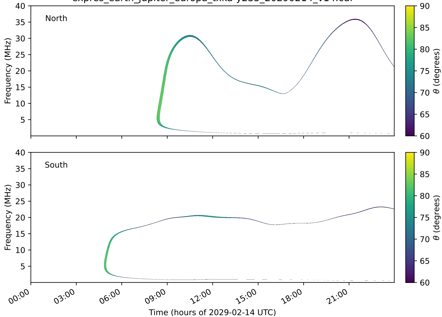
expres_earth_jupiter_europa_txka-y235_20290214_v14.cdf
