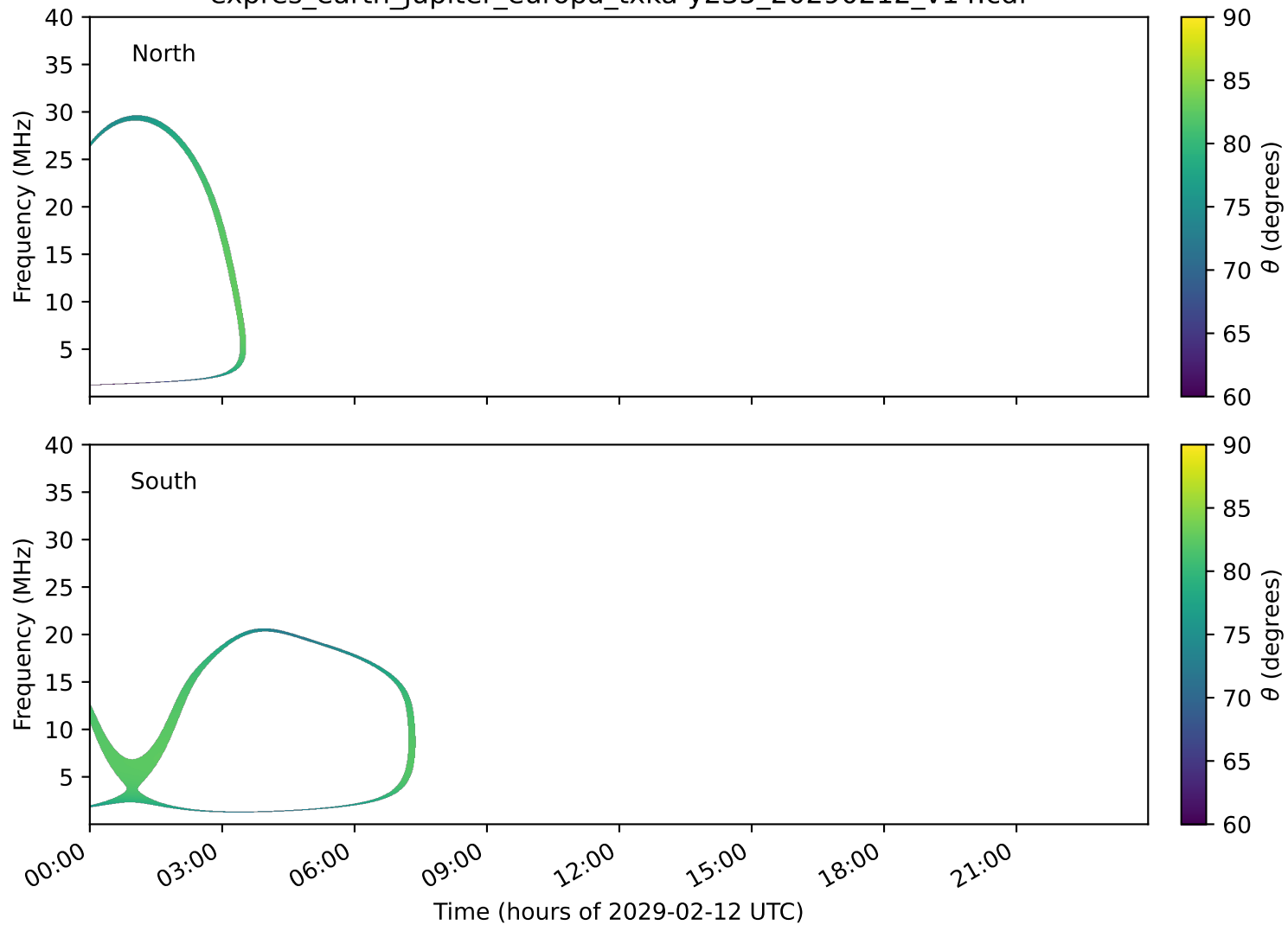
expres_earth_jupiter_europa_txka-y235_20290212_v14.cdf
