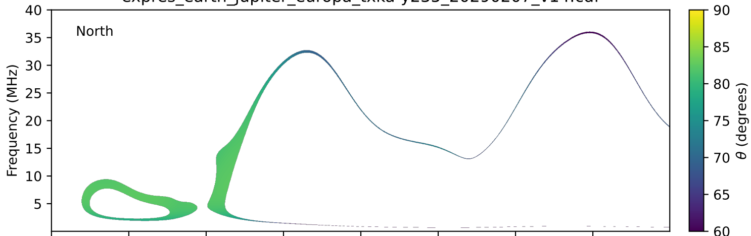
expres_earth_jupiter_europa_txka-y235_20290207_v14.cdf
