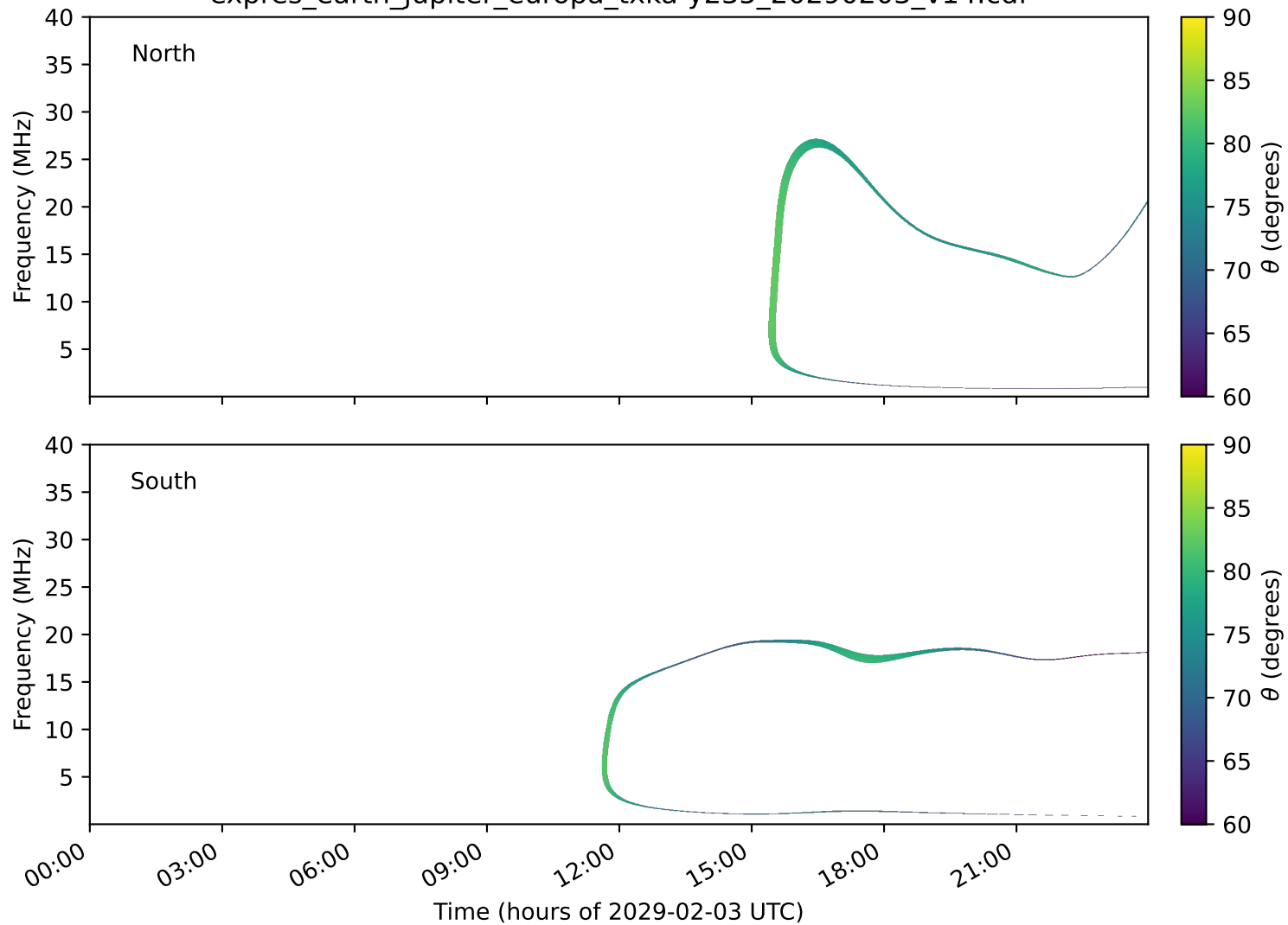
expres_earth_jupiter_europa_txka-y235_20290203_v14.cdf
