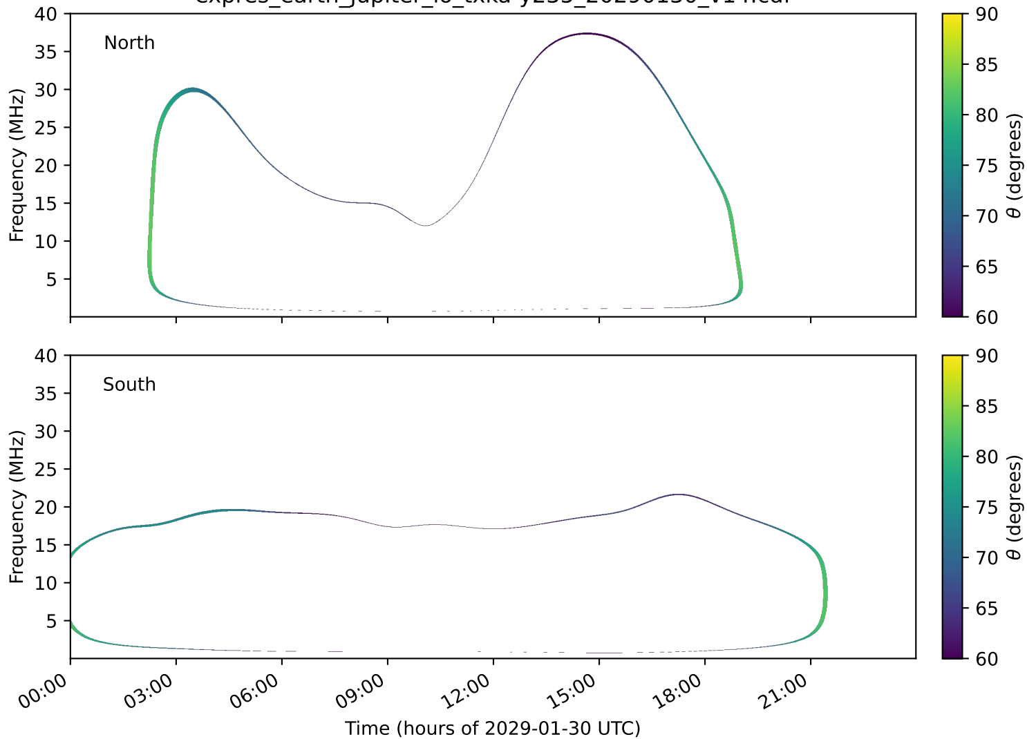
expres_earth_jupiter_io_txka-y235_20290130_v14.cdf
