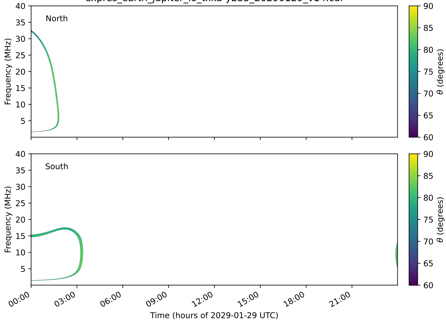
expres_earth_jupiter_io_txka-y235_20290129_v14.cdf
