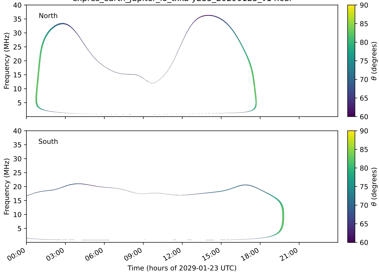
expres_earth_jupiter_io_txka-y235_20290123_v14.cdf
