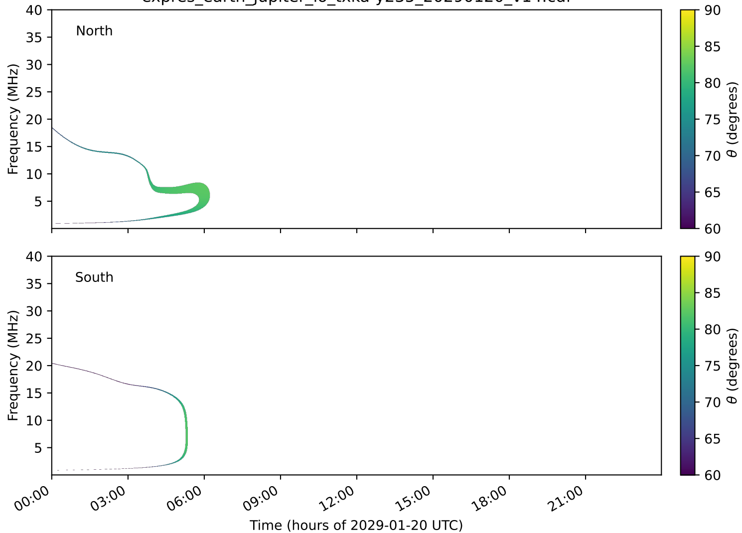
expres_earth_jupiter_io_txka-y235_20290120_v14.cdf
