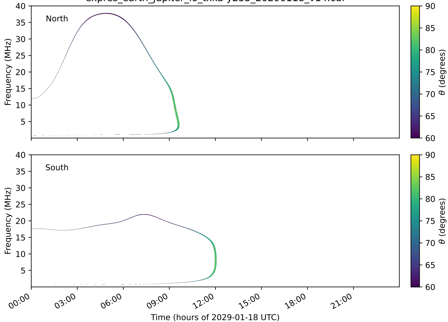
expres_earth_jupiter_io_txka-y235_20290118_v14.cdf
