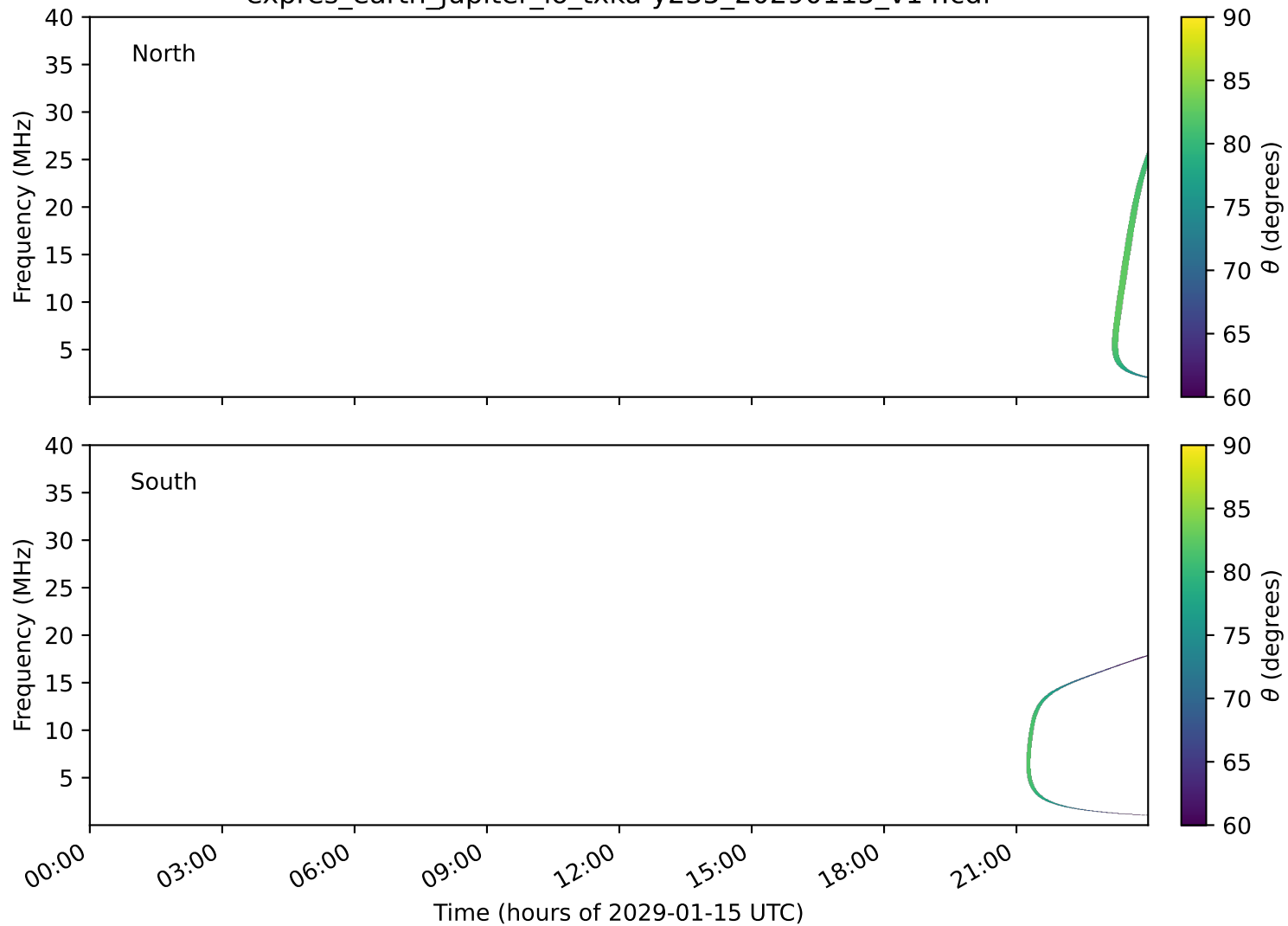
expres_earth_jupiter_io_txka-y235_20290115_v14.cdf
