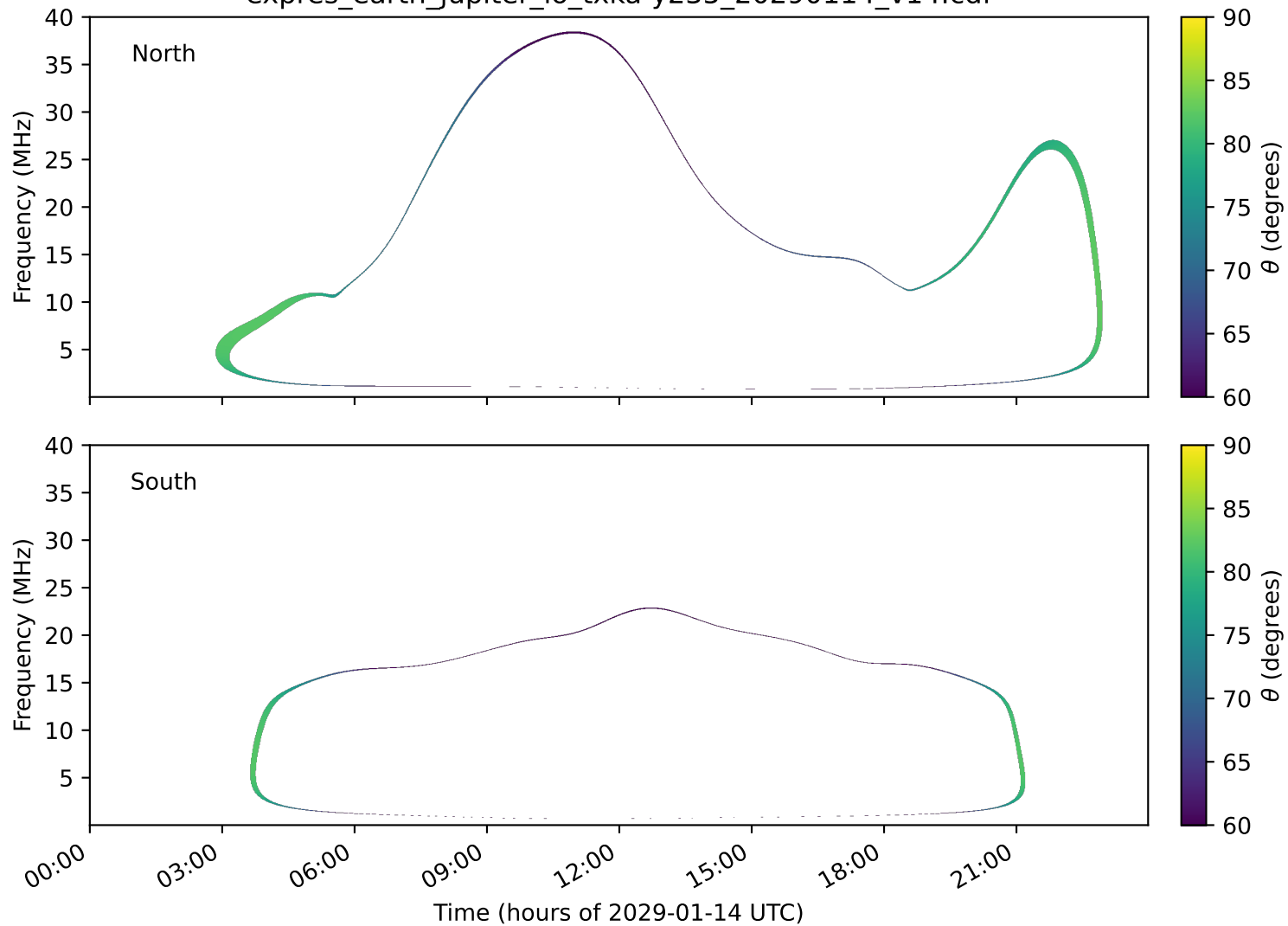
expres_earth_jupiter_io_txka-y235_20290114_v14.cdf
