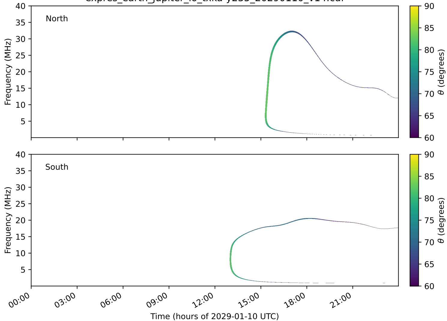
expres_earth_jupiter_io_txka-y235_20290110_v14.cdf
