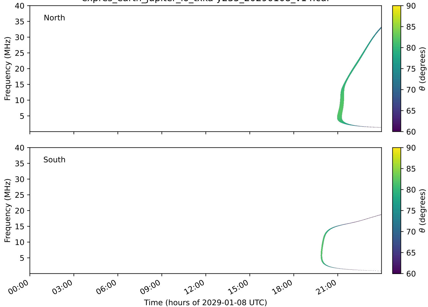
expres_earth_jupiter_io_txka-y235_20290108_v14.cdf
