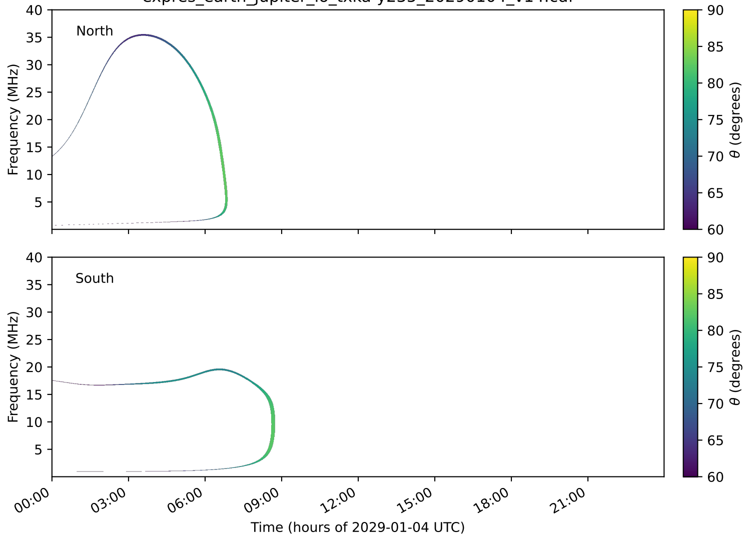
expres_earth_jupiter_io_txka-y235_20290104_v14.cdf
