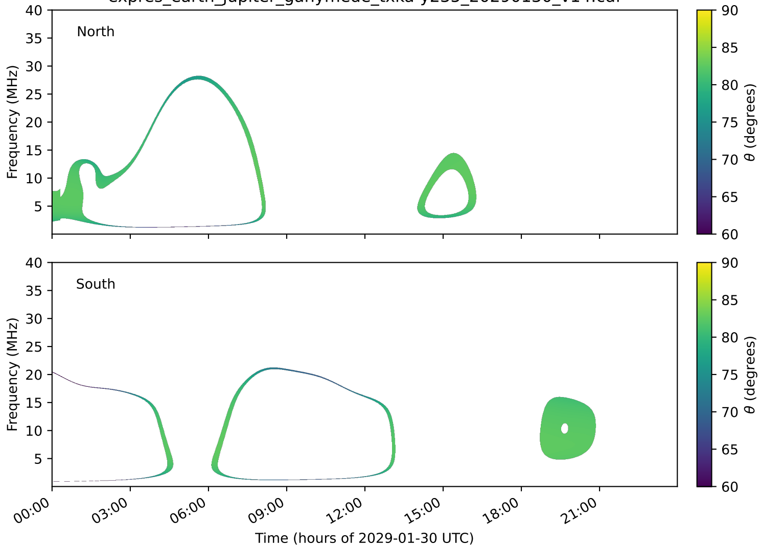
expres_earth_jupiter_ganymede_txka-y235_20290130_v14.cdf
